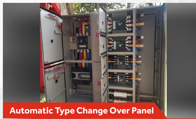
ATS Enclosure (Auto Transfer Switch)
